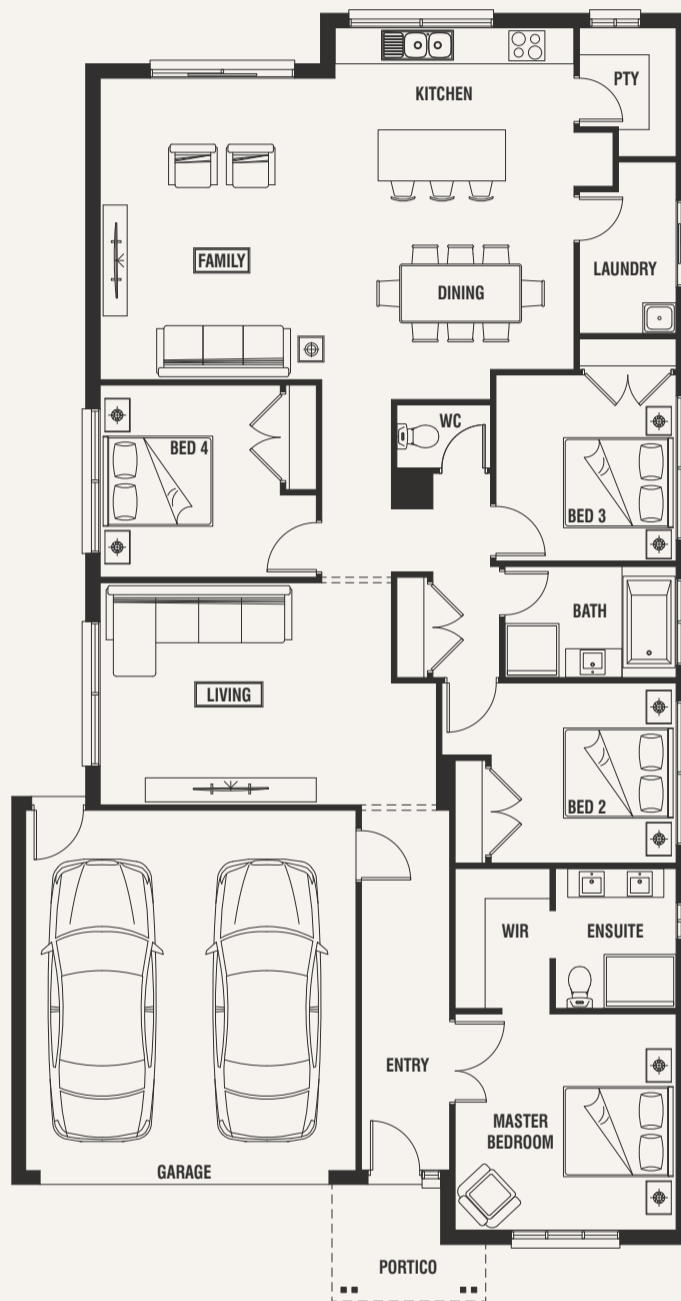
Standard floorplan with Riva façade
