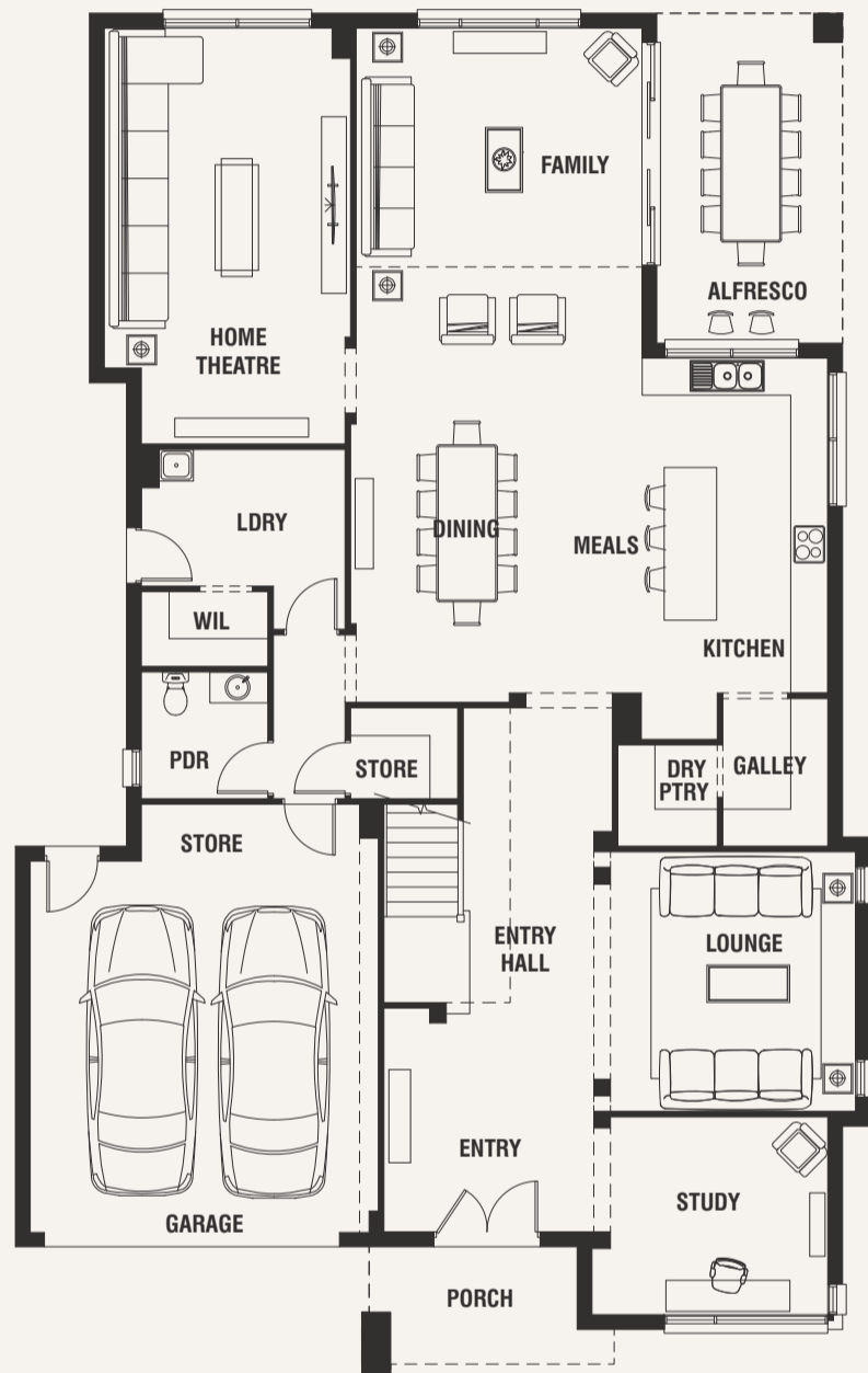
Standard floorplan with Retro façade
